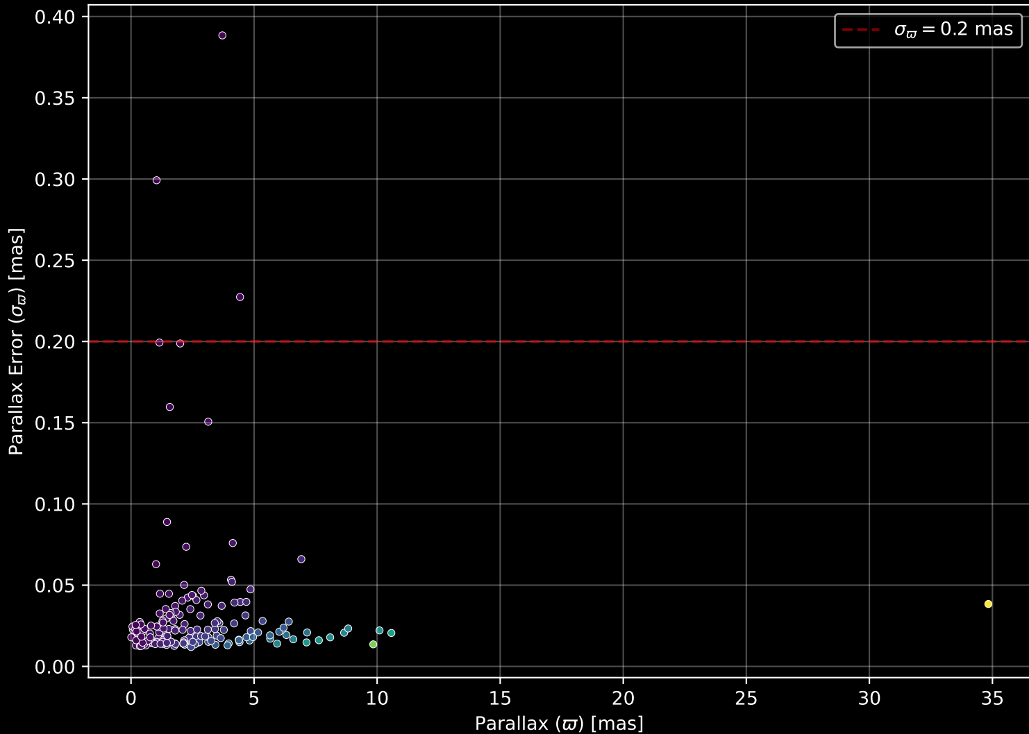
APOGEE DR17 Field: [172+58_btx] Parallax Quality (n= 182)
