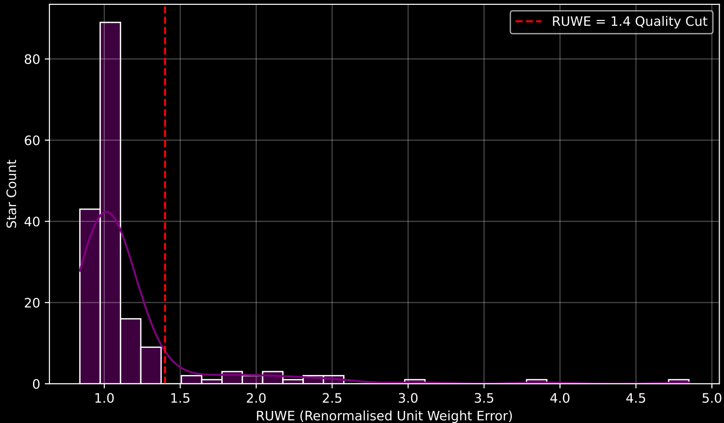
GAPOGEE DR17 Field [172+58_btx] RUWE Distribution (n= 176)
