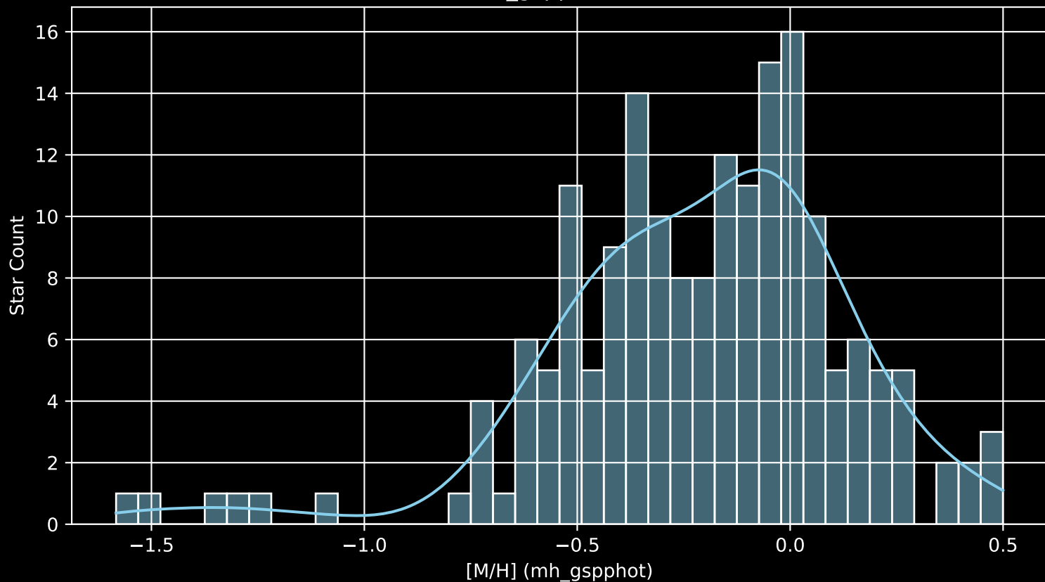
APOGEE DR17 Field: [172+58_btx [M/H] (mh_gspphot) (n= 180)
