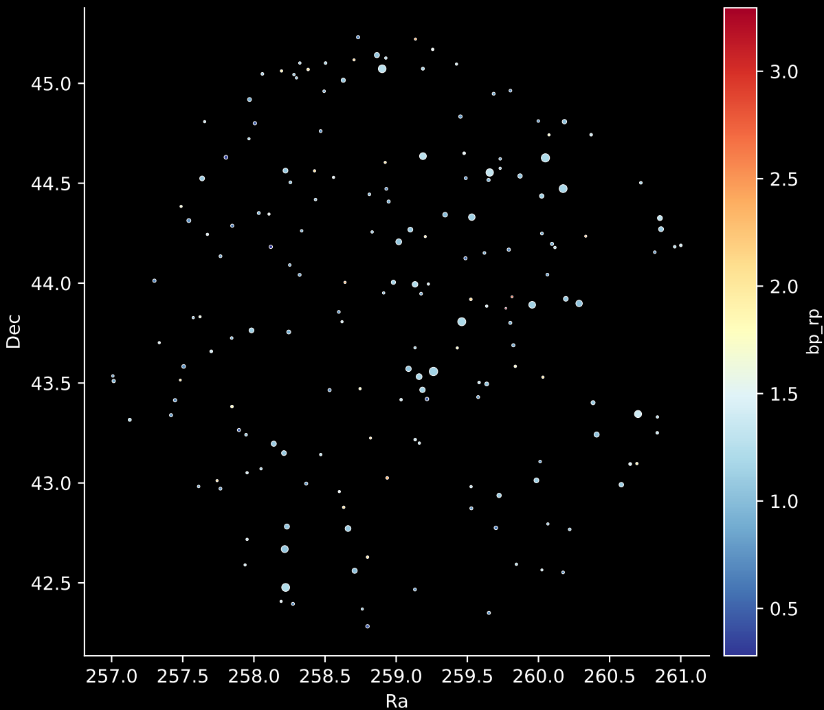
APOGEE DR17 Field: [172+58_btx] Stars: 182
