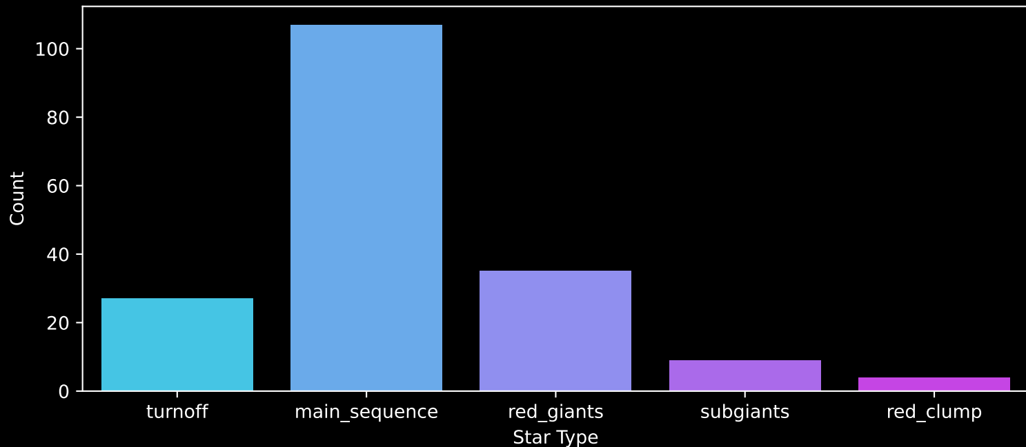
APOGEE DR17 Field: [172+58_btx] Count plot of Star Type
