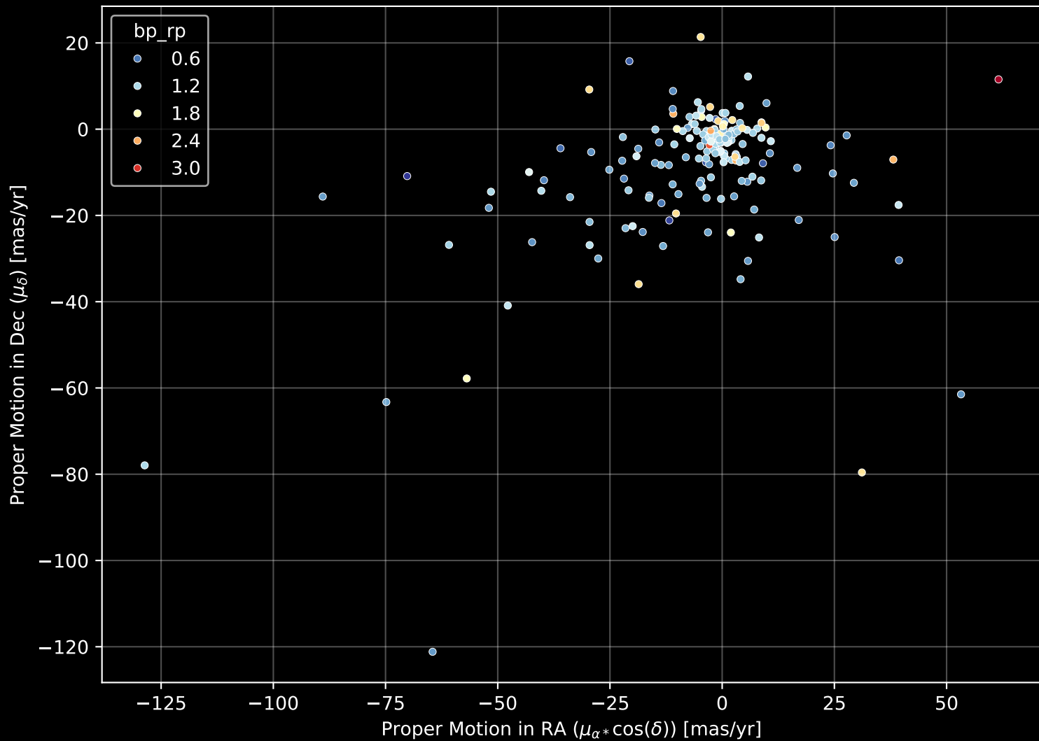
APOGEE DR17 Field: [172+58_btx] Proper Motion Diagram (n= 182)
